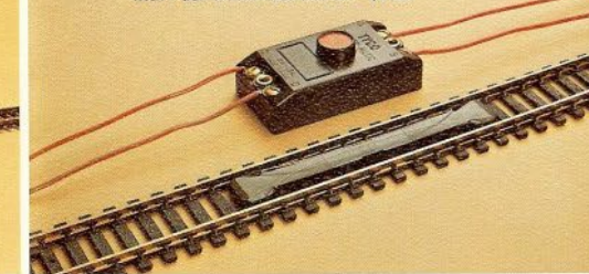
No. 923 — REMOTE CONTROL UNCOUPLING TRACK, Complete with Push-button Controller $3.00
