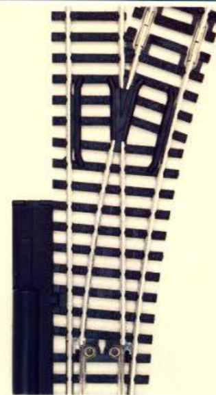
No. 464—2-way remote control switch No. 415—90° track crossing No. 970—Blocking switch, with 4 insulated rail joiners
